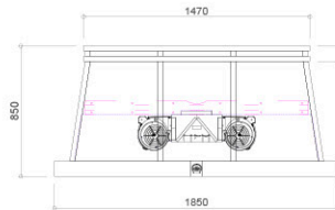
Hotte Château 165: H18T0SM 1850 W x 850 H x 650 D (mm) 72.8 W x 33.5 H x 25.6 D (inches) Motorized Hood Starting from $28,500
