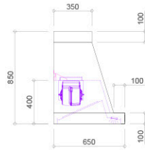
Standard Configuration Motorized Wall Hood Side View
