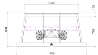
Hotte Château 150: H17T0SM 1700 W x 850 H x 650 D (mm) 66.9 W x 33.5 H x 25.6 D (inches) Motorized Hood Starting from $26,400
