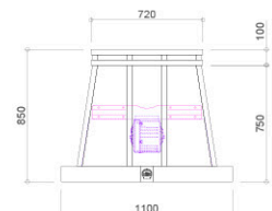
Hotte Château 90: H11T0SM 1100 W x 850 H x 650 D (mm) 43.3 W x 33.5 H x 25.6 D (inches) Motorized Hood Starting from $20,700
