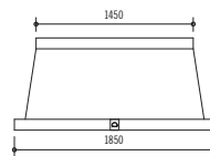
Hotte Château 165: H18TO 1850 W x 850 H x 650 D (mm) 72.8 W x 33.5 H x 25.6 D (inches) Shell-Only Starting from $16,000 Motorized Hood Starting from $20,200 Island configuration: H18CO Starting from $27,500
