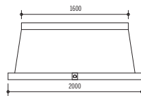
Hotte Grand Palais 180: H20TO 2000 W x 850 H x 650 D (mm) 78.7 W x 33.5 H x 25.6 D (inches) Shell-Only Starting from $17,100 Motorized Hood Starting from $21,300 Island configuration: H20CO Starting from $29,300
