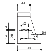
Standard Configuration Motorized Wall Hood Side View
