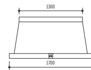
Hotte Château 150: H17TO 1700 W x 850 H x 650 D (mm) 66.9 W x 33.5 H x 25.6 D (inches) Shell-Only Starting from $15,000 Motorized Hood Starting from $18,800 Island configuration: H17CO Starting from $25,800
