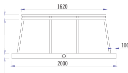
Hotte Grand Palais 180: H20T0S M 2000 W x 850 H x 650 D (mm) 78.7 W x 33.5 H x 25.6 D (inches) Motorized Hood Starting from $25,600
