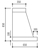
Standard Configuration Wall Hood Side View
