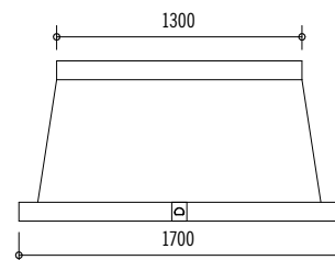
Standard Configuration Island Hood Side View
