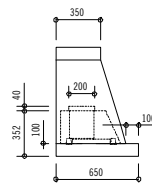
Standard Configuration Motorized Wall Hood Side View
