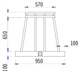
Hotte Château 75: H95T0S M 950 W x 850 H x 650 D (mm) 37.4 W x 33.5 H x 25.6 D (inches) Mortorized Hood Starting from $13,200
