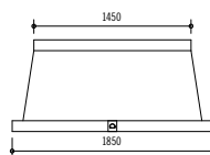
Hotte Château 165: H18T0 1850 W x 850 H x 650 D (mm) 72.8 W x 33.5 H x 25.6 D (inches) Shell-Only Starting from $12,200 Motorized Hood Starting from $15,500 Island configuration: H18C0 Starting from $21,000 Motorized Island Hood Starting from: $22,400
