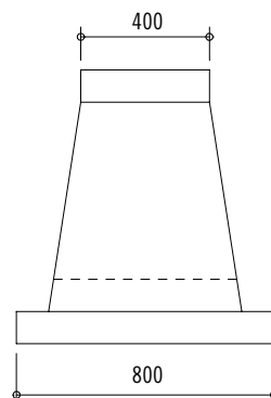
Standard Configuration Island Hood Side View
